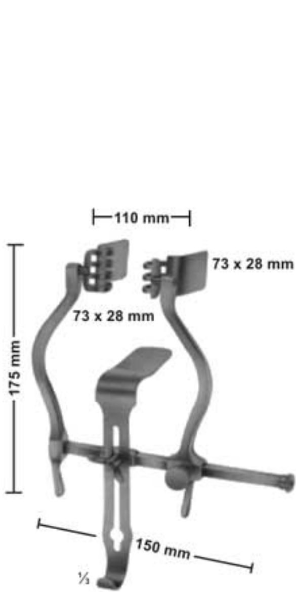
09-101 JUDD-MASSON Bladder-and suprapubic retractor
